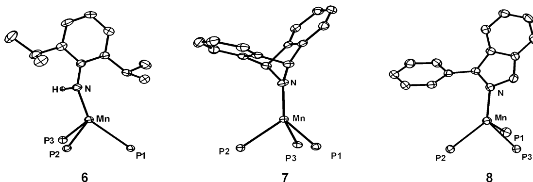
Figure 6. Displacement ellipsoid representations (50%) of [\text{PhBP}^{\text{iPr}}_3]\text{Mn}(\text{NH}(2,6\text{-iPr}_2\text{-C}_6\text{H}_3)) ( 6 ), [\text{PhBP}^{\text{iPr}}_3]\text{Mn}(\text{dbabh}) ( 7 ), and [\text{PhBP}^{\text{iPr}}_3]\text{Mn}(1\text{-Ph(isoindolate)}) ( 8 ). For clarity, hydrogen atoms (except N-H) have been omitted and only the phosphorus atoms of the ligand are shown. Selected bond distances (Å) and angles (deg) for 6 : Mn–N 1.997(2), Mn–P1 2.5877(6), Mn–P2 2.5813(6), Mn–P3 2.5637(6), P1–Mn–P2 87.96(2), P2–Mn–P3 89.95(2), P1–Mn–P3 93.11(2), N–Mn–P1 144.77(5), N–Mn–P2 105.73(5), N–Mn–P3 118.63(5). For 7 : Mn–N 1.948(1), Mn–P1 2.5357(5), Mn–P2 2.5473(5), Mn–P3 2.5503(5), P1–Mn–P2 90.46(2), P2–Mn–P3 89.51(2), P1–Mn–P3 90.71(2), N–Mn–P1 126.19(4), N–Mn–P2 126.13(4), N–Mn–P3 122.92(4). For 8 : Mn–N 2.054(2), Mn–P1 2.5308(7), Mn–P2 2.5550(7), Mn–P3 2.5718(6), P1–Mn–P2 95.13(2), P1–Mn–P3 89.54(2), P2–Mn–P3 90.09(2), N–Mn–P1 111.98(5), N–Mn–P2 136.31(5), N–Mn–P3 122.30(5).
