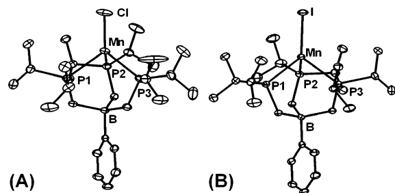
Figure 1. Displacement ellipsoid representations (50%) of (A) [PhBP i Pr 3 ]-MnCl ( 1a ) and (B) [PhBP i Pr 3 ]-MnI ( 2 ). Hydrogen atoms and solvent molecules have been omitted for clarity. Selected bond distances (Å) and angles (deg) for 1a : Mn–Cl 2.2687(7), Mn–P1 2.5300(6), Cl–Mn–P1 125.38(2), Mn–P2 2.5298(6), Mn–P3 2.5289(6), Cl–Mn–P2 120.22(2), Cl–Mn–P3 126.14(2), P1–Mn–P2 90.55(2), P2–Mn–P3 92.64(2), P1–Mn–P3 92.22(2). For 2 : Mn–I 2.6394(4), Mn–P1 2.5351(7), Mn–P2 2.5238(7), Mn–P3 2.5379(6), P1–Mn–I 127.19(2), P2–Mn–I 122.27(2), P3–Mn–I 124.09(2), P1–Mn–P2 91.39(2), P2–Mn–P3 90.68(2), P1–Mn–P3 90.95(2).
