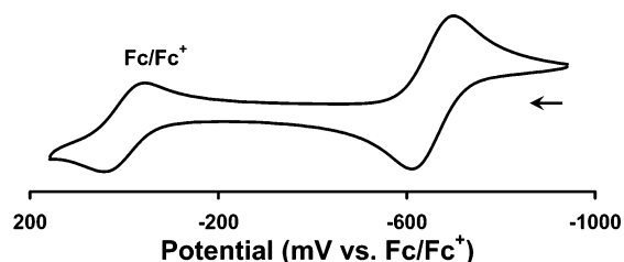
Figure 10. Cyclic voltammogram of [PhBP i Pr 3 ]Mn(CN t Bu) 3 ( 10 ) recorded at a scan rate of 100 mV/s in THF with 0.35 M [ n Bu 4 ][PF 6 ] as the supporting electrolyte. Potentials are internally referenced to Fc/Fc + .
