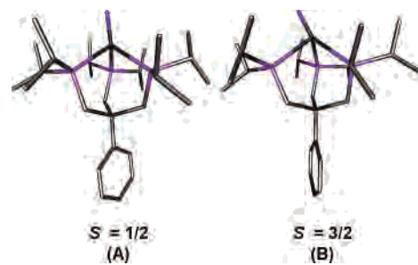
Figure 12. DFT-optimized structures (Jaguar 5.0, B3LYP/LACVP**) for (A) doublet [\text{PhBP}^{i\text{Pr}}_3]\text{Mn}(\text{N}) and (B) quartet [\text{PhBP}^{i\text{Pr}}_3]\text{Mn}(\text{N}) . Selected bond distances (Å) and angles (deg) for (A): Mn–N 1.50; Mn–P 2.35, 2.41, 2.45; N–Mn–P 112.1, 122.3, 127.5; P–Mn–P 94.8, 95.6, 97.2. For (B): Mn–N 1.62; Mn–P 2.48, 2.49, 2.60; N–Mn–P 103.9, 109.3, 155.3; P–Mn–P 89.9, 90.5, 91.2.
