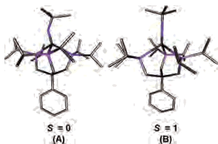
Figure 11. DFT-optimized structures (Jaguar 5.0, B3LYP/LACVP**) for (A) singlet [\text{PhBP}^{i\text{Pr}}_3]\text{Mn}(\text{N}'\text{Bu}) and (B) triplet [\text{PhBP}^{i\text{Pr}}_3]\text{Mn}(\text{N}'\text{Bu}) . Selected bond distances (Å) and angles (deg) for (A): Mn–N 1.63; Mn–P 2.28, 2.36, 2.36; Mn–N–C 144.8; P–Mn–P 96.8, 97.2, 97.7; N–Mn–P 104.7, 126.2, 127.2. For (B): Mn–N 1.66; Mn–P 2.40, 2.44, 2.45; Mn–N–C 179.2; P–Mn–P 89.5, 89.8, 91.5; N–Mn–P 121.9, 126.2, 127.0.
