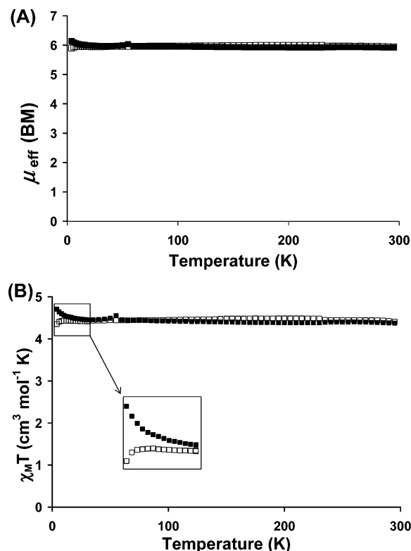
Figure 3. (A) SQUID plot of \mu_{\text{eff}} ( \mu_{\text{B}} ) versus T and (B) \chi_{\text{M}}T ( \text{cm}^3\text{K/mol} ) versus T for [\text{PhBP}^{\text{iPr}}_3]\text{MnCl} , 1 , (■), and [\text{PhBP}^{\text{iPr}}_3]\text{MnI} , 2 , (□). An expansion of the \chi_{\text{M}}T vs T plot at low temperatures (4–30 K) is shown in the inset.
