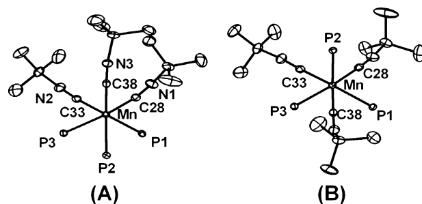
Figure 9. Displacement ellipsoid representations (50%) of [PhBP i Pr 3 ]Mn–(CN t Bu) 3 ( 10 ) from the side (A) and top (B) views. For clarity, hydrogen atoms have been omitted and only the phosphorus atoms of the ligand are shown. Selected bond distances (Å) and angles (deg) for 10 : Mn–C28 1.870(1), Mn–C33 1.864(1), Mn–C38 1.835(1), N1–C28 1.176(2), N2–C33 1.176(2), N3–C38 1.185(2), Mn–P1 2.3597(4), Mn–P2 2.3831(4), Mn–P3 2.3655(3), P1–Mn–P2 88.59(1), P2–Mn–P3 86.49(1), P1–Mn–P3 89.17(1), C33–Mn–C28 83.75(5), C38–Mn–C28 85.26(5), C38–Mn–C33 89.12(5).
