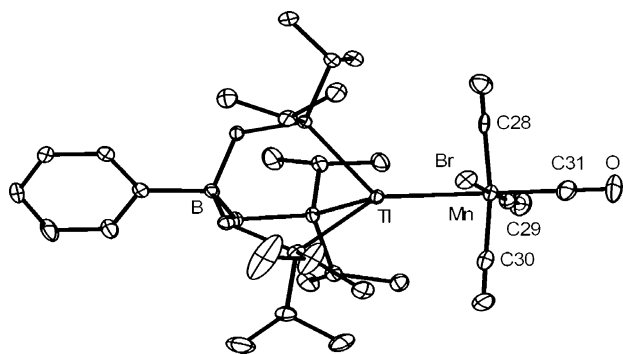
Figure 8. Displacement ellipsoid representations (50%) of [PhBP i Pr 3 ]Ti–MnBr(CO) 4 ( 9 ). For clarity, hydrogen atoms have been omitted. Selected bond distances (Å) and angles (deg) for 9 : Mn–Ti 2.6437(4), Mn–C28 1.913(3), Mn–C29 1.799(3), Mn–C30 1.851(3), Mn–C31 1.823(3), Mn–Br 2.5299(4), C31–Mn–Ti 172.74(8), Br–Mn–Ti 86.11(1), C29–Mn–C28 92.6(1), C29–Mn–C30 91.1(1), C28–Mn–Br 85.39(7), C29–Mn–Br 177.98(8), C30–Mn–Br 90.94(8), C31–Mn–Br 86.73(8).
